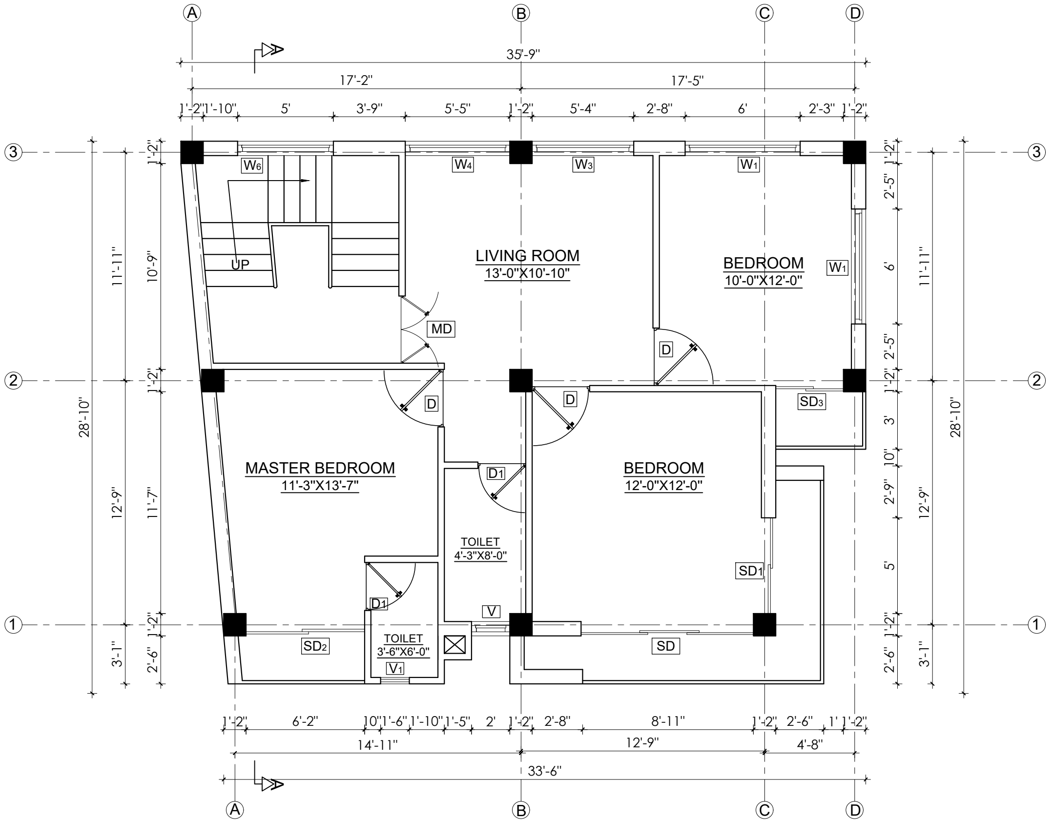
FIRST FLOOR PLAN AREA=848.81 SQ.FT.
